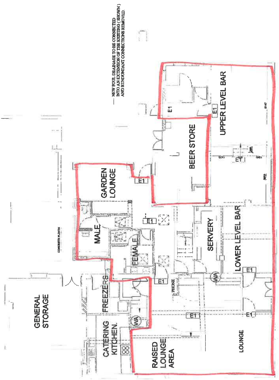
GROUND FLOOR PLAN AS PROPOSED - CHECK SURVEY
